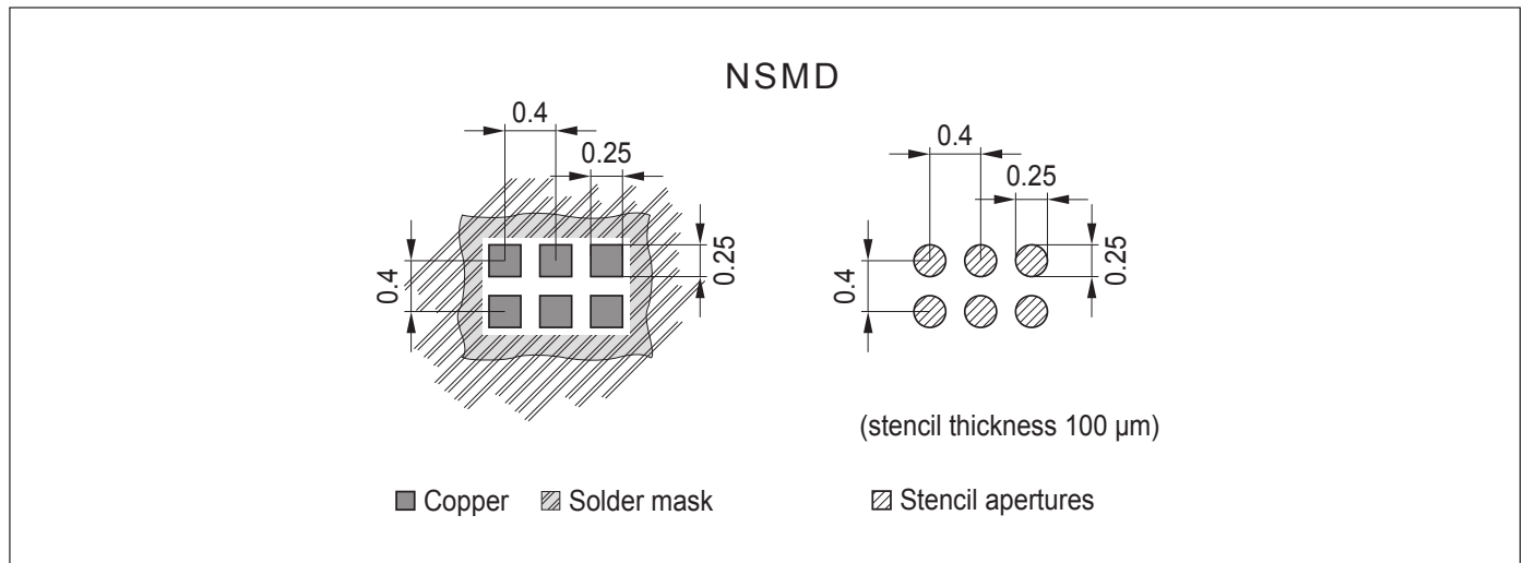
Figure 4: Footprint Recommendation
